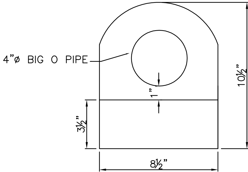
END PROFILE
